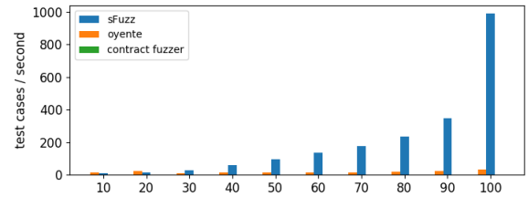
Figure 5: Efficiency comparison between sFuzz, Oyente, and ContractFuzzer
