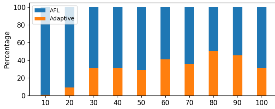
Figure 9: Percentage of test cases due to adaptive strategy
